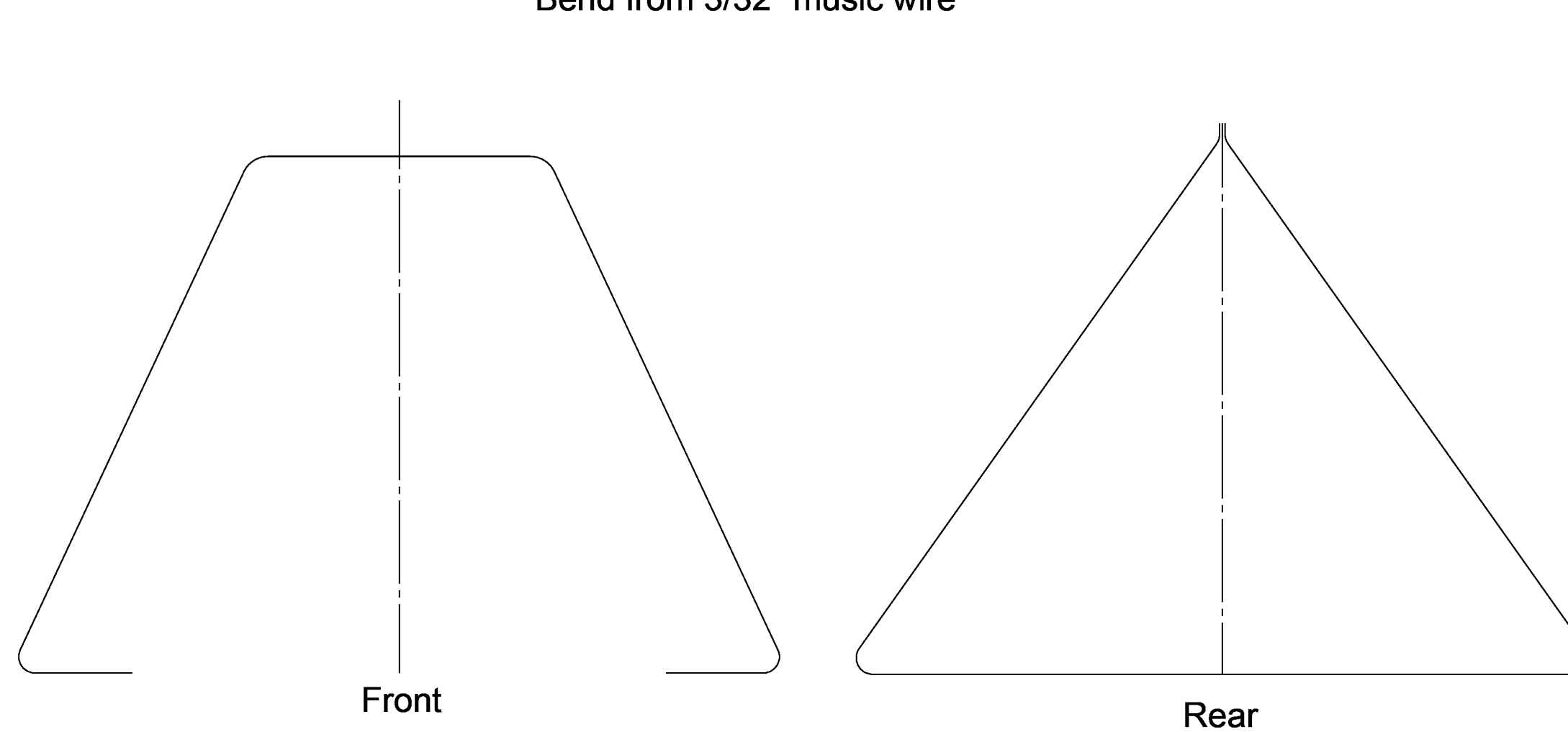
Landing Gear Strut Bend Templates
